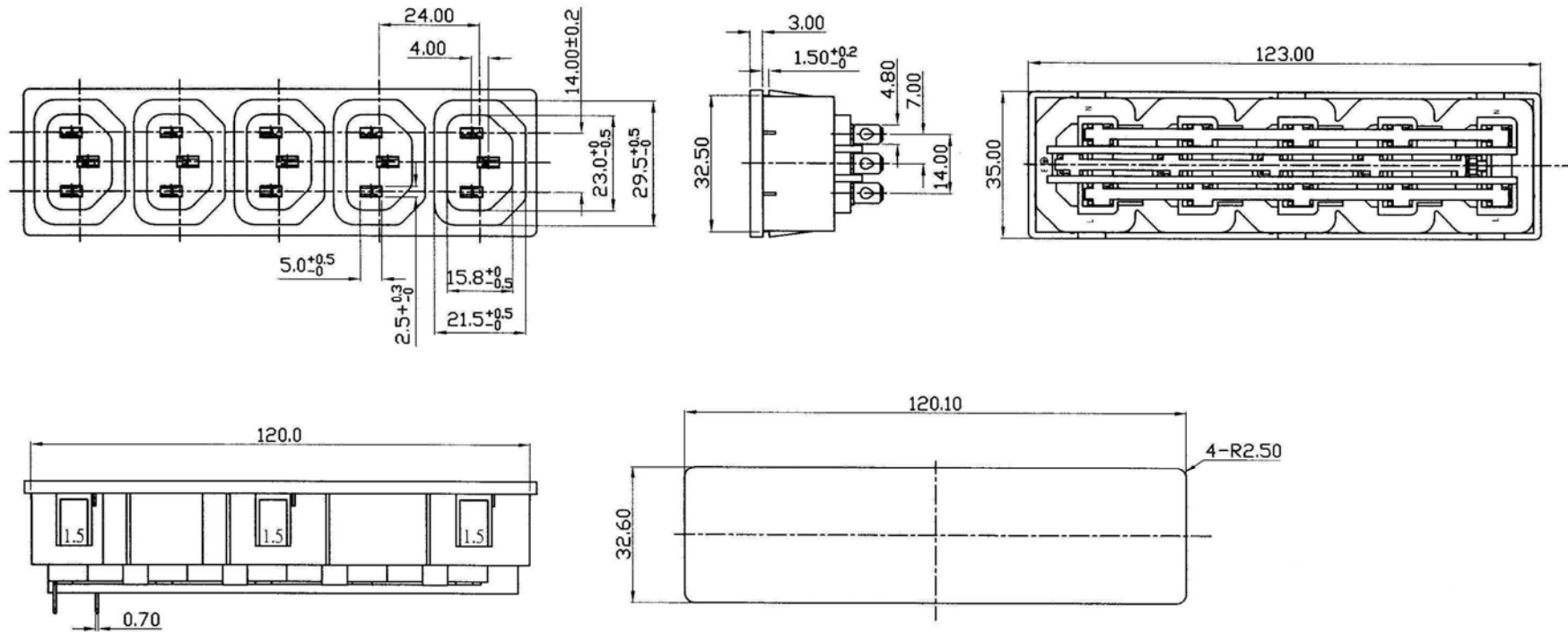
PANEL CUT-OUT
