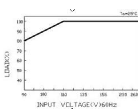
Static Characteristics (5V)
