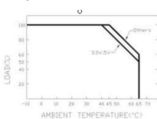
Derating Curve
